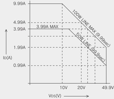
Forcing Power Range Diagram
