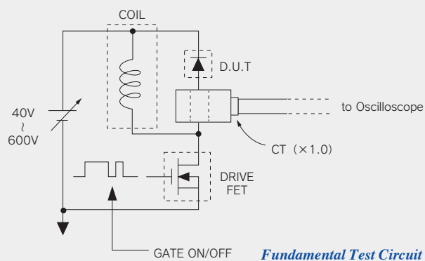
Fundamental Test Circuit
