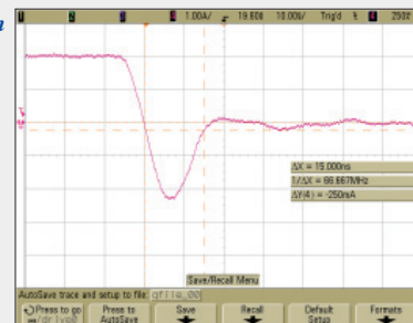
Measurement Waveform
